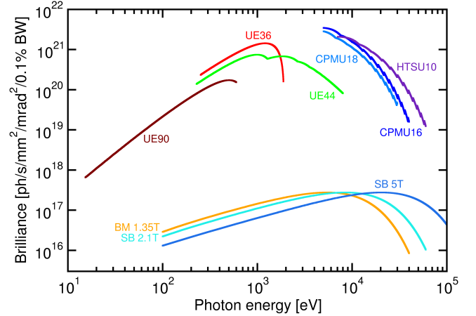
Figure 6. Brilliance curves of the SLS 2.0 sources. CPMU = cryogenic permanent-magnet undulator; HTSU = high-temperature superconducting undulator; UE = elliptical undulator; two-digit suffices = undulator periodicity in mm. BM = bending magnet; SB = superbend; field strengths in Tesla.
