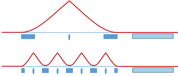
Figure 2. Schematics of a double bend achromat (DBA) and multi-bend achromat (MBA). The red line indicates the dispersion, which is refocused by magnetic lenses (quadrupoles) in order to minimize it inside the dipoles and to suppress it in the straight sections, where the undulators are located.
