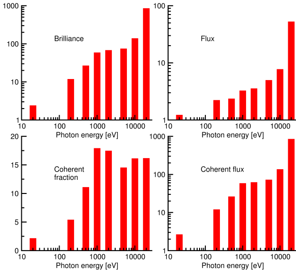
Figure 10. Improvement factors in brilliance, flux, coherent fraction, and coherent flux for the SLS 2.0 upgrade compared to the present SLS, with the new storage-ring energy of 2.7 GeV, for selected photon energies. The undulators assumed in the original SLS are UE212 (8.4 m) for 20 and 200 eV, UE56 (3.6 m) for 500, 1000, and 2000 eV, and U19 (1.8 m) for higher photon energies. The corresponding undulators in SLS 2.0 are UE90 (4.4 m), UE36 (4.4 m), and CPMU15 (3 m).
