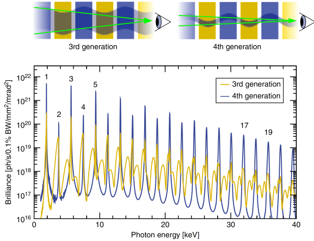
Figure 7. Comparison of the brilliance of undulator spectra at third- and fourth-generation facilities. Top: the width of the electron beam passing through an undulator at third-generation facilities is approximately two orders of magnitude larger than the oscillation amplitude, while at DLSRs, it might only be approximately ten times, or even less. Bottom: consequently, less off-axis radiation (given by Equation 10) is produced by undulators at DLSRs. Note also the enhanced brilliance at the spectral peaks for the DLSR. Both simulated spectra were generated for a U12 undulator (that is, \lambda_u = 12 mm) containing 120 magnet periods, for K = 1.6 , 400 mA, and a storage-ring energy, currently used at SLS, of 2.4 GeV. Adapted from [8] with permission from John Wiley & Sons.
