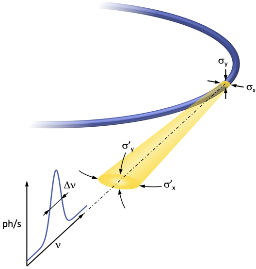
Figure 1. Schematic of the parameters determining brilliance, see Equation 1. The root-mean-square (RMS) source sizes ( \sigma_{x,y} ) and divergences ( \sigma'_{x,y} ) in the planes perpendicular to the direction of radiation define the emittance; the relative bandwidth is given by the bandwidth \Delta\nu divided by the central frequency \nu , a delivering a flux given in \text{ph s}^{-1} .
