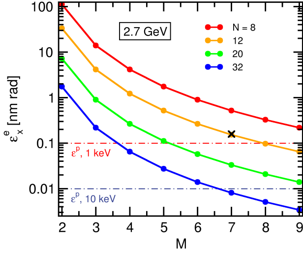
Figure 4. Plot of the theoretically optimal horizontal electron emittance \varepsilon_x^e as a function of the number of straights N in a 2.7-GeV synchrotron ring and number of dipoles M within a single arc sector, according to Equation 6. Values for N = 12, 20 , and 32 were selected, as these correspond to SLS 2.0, MAX-IV, and ESRF-EBS, respectively. Also included as dot-dash lines are the fundamental photon emittances for 1 and 10-keV photons, given by Equation 4, and the position of SLS 2.0, labelled as the black X.
