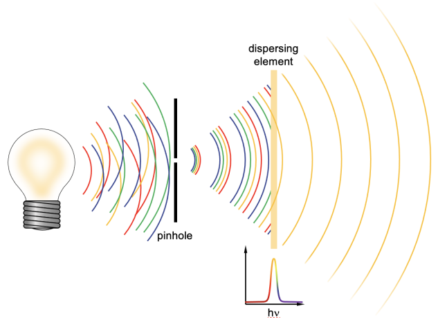
Figure 5. Coherent radiation can be extracted from a broadband, spatially extended source by the use of a pinhole and a dispersive element that selects a narrow band of wavelengths.
