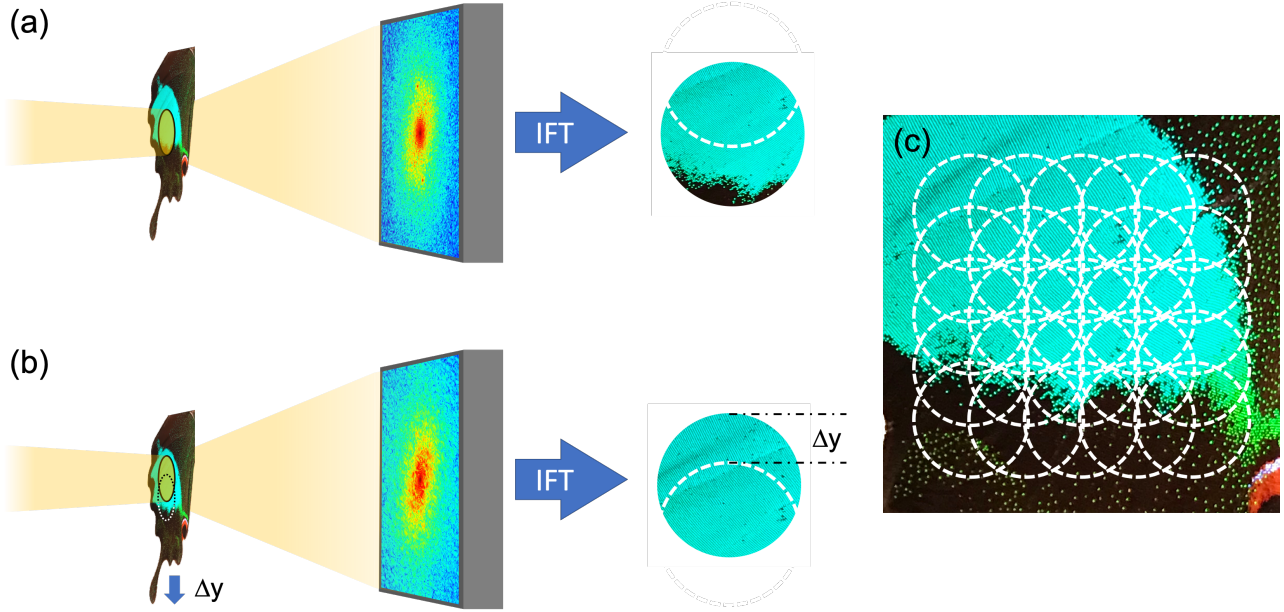
Figure 9. Principle of image reconstruction in ptychography. (a) An object is locally illuminated and the forward-scattered radiation is captured on an x-ray detector. If the phases of the individual amplitudes (these being proportional to the square root of the recorded intensity in each pixel) are correctly chosen, the inverse Fourier transform (IFT) will yield a real-space image of the region of the sample which was illuminated. (b) The sample is moved through a distance \Delta y which is smaller than the illumination diameter, and the next scattering pattern is recorded and IFT calculated. The region common to the first and second illuminations (i.e., the region encompassed by the dashed circle and the edge of the image) should thus be identical. It is this condition which is used to ensure that the phases have been correctly chosen, through an iterative algorithm [24]. (c) By scanning the sample over a large area and recording the scattering pattern at each step, very large volumes of the object can be reconstructed, limited only by the computer power and storage capacity on the one hand, and the dosage on the other.
