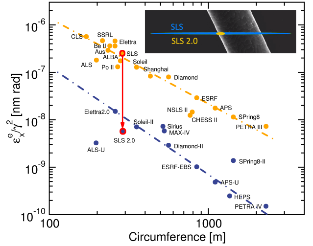
Figure 3. Plot of horizontal electron emittances weighted by the square of the storage-ring energy as a function of ring circumference (see Equation 5), for both a selection of third- (orange data points) and fourth-generation (blue) synchrotrons. Note the approximately fortyfold improvement in the weighted emittance for the SLS 2.0 upgrade, highlighted in red. The inset shows the cross-sections of the electron beams at SLS and SLS 2.0 compared to a typical human hair.
